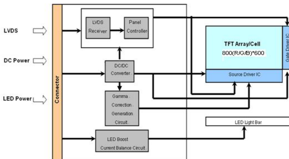
Figure 1 Block Diagram
